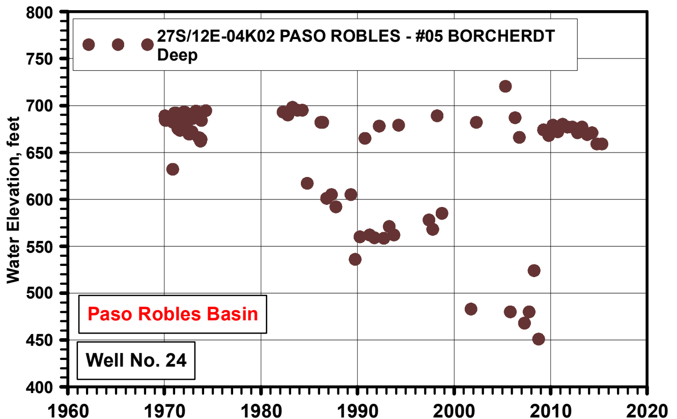
HYDROGRAPHS 17 AND 24
