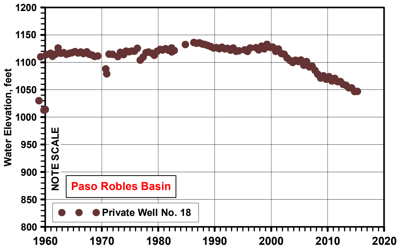
HYDROGRAPHS 11 AND 18
